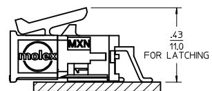
SECTION "A"- "A" WITH TERMINAL SCALE 10:1
